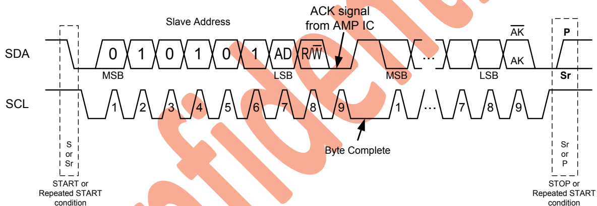
Figure 3. Basic Signaling Elements of I 2 C Bus
